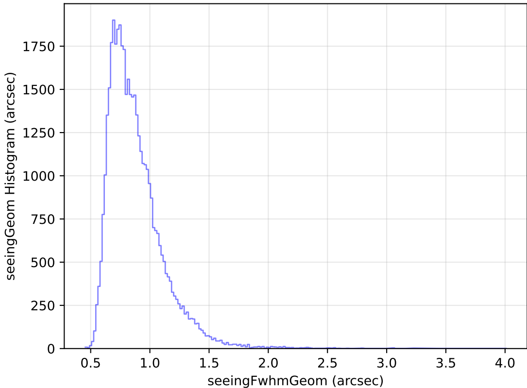
weather_cloudso6v3.4_10yrs Yr 1 z band: seeingGeom Histogram
