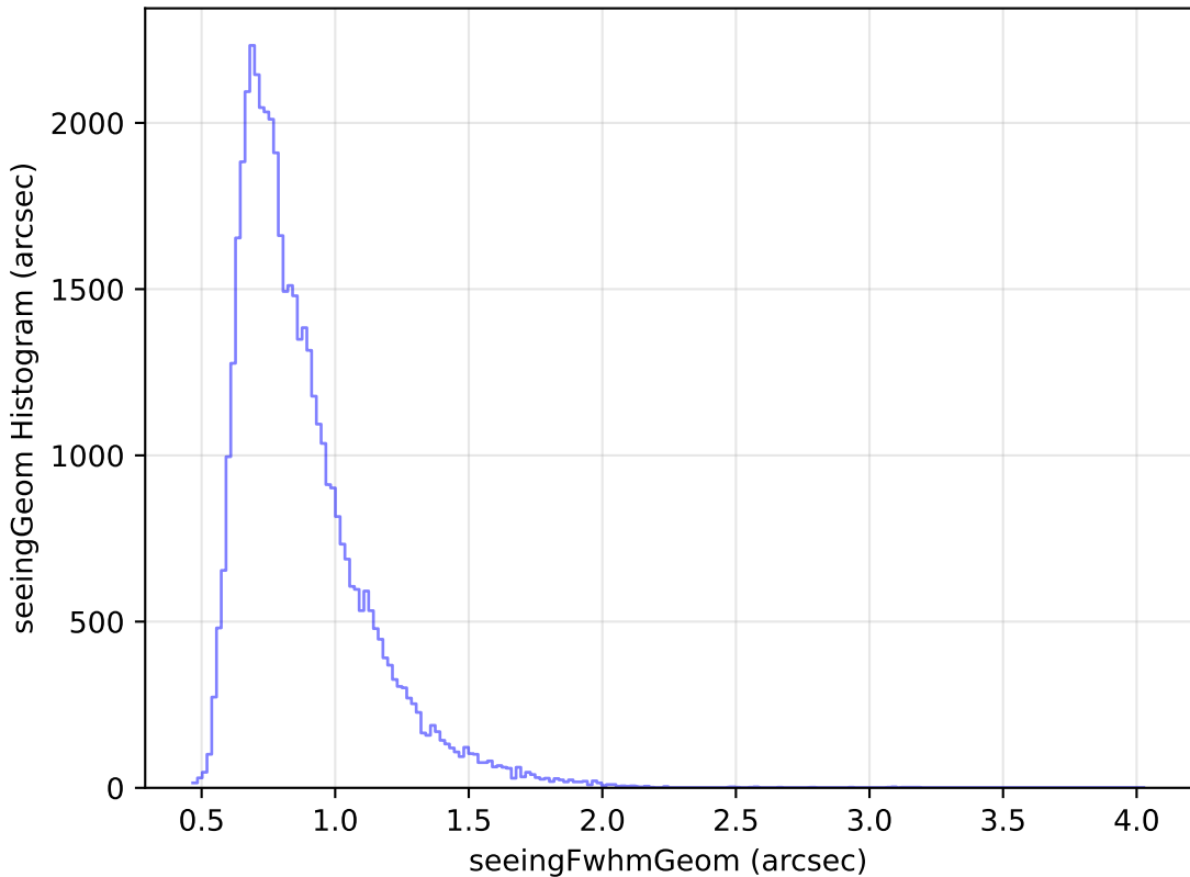
weather_cloudso6v3.4_10yrs Yr 1 r band: seeingGeom Histogram
