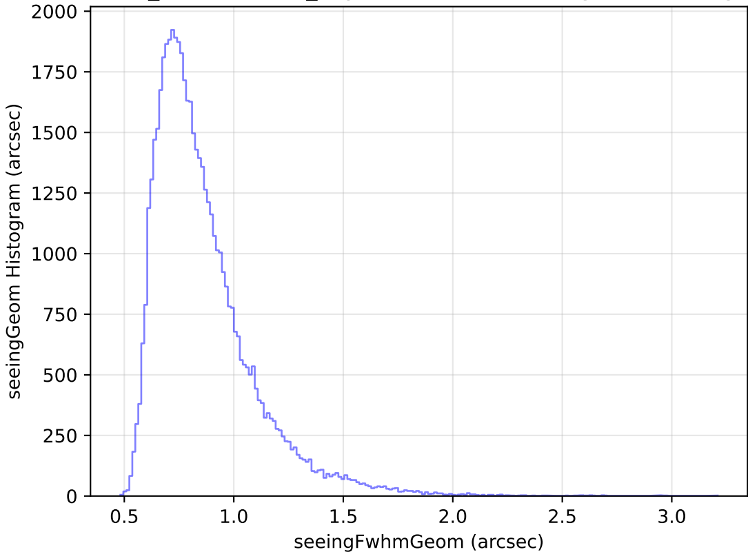
weather_cloudso6v3.4_10yrs Yr 1 i band: seeingGeom Histogram
