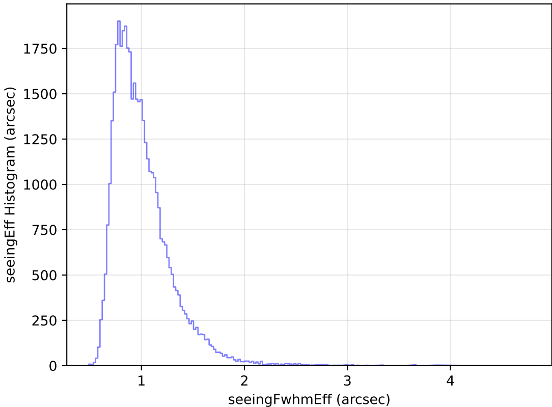
weather_cloudso6v3.4_10yrs Yr 1 z band: seeingEff Histogram
