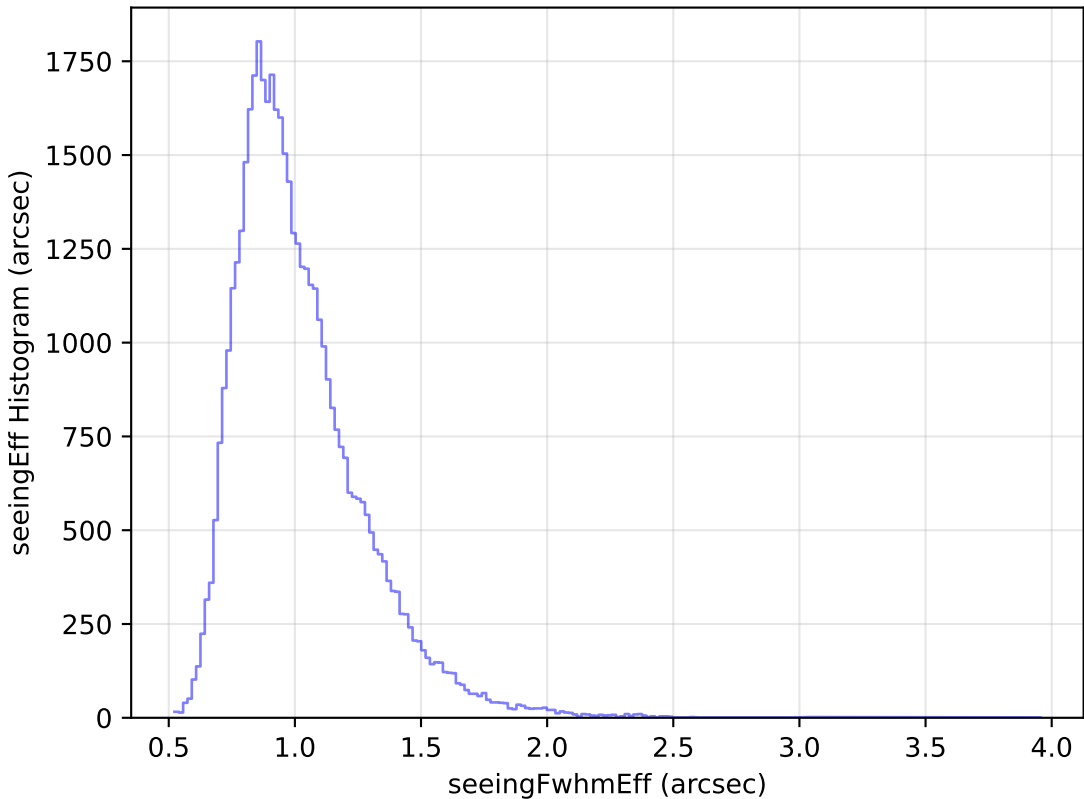
weather_cloudso6v3.4_10yrs Yr 1 y band: seeingEff Histogram
