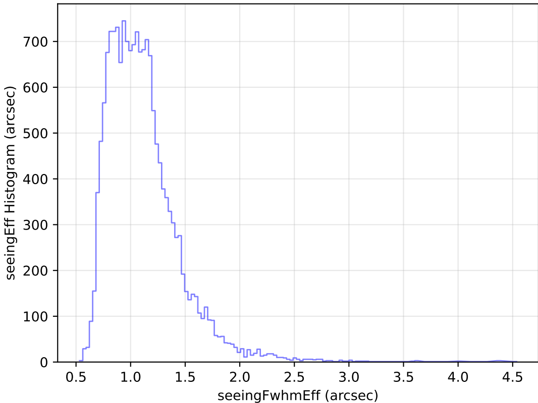
weather_cloudso6v3.4_10yrs Yr 1 u band: seeingEff Histogram
