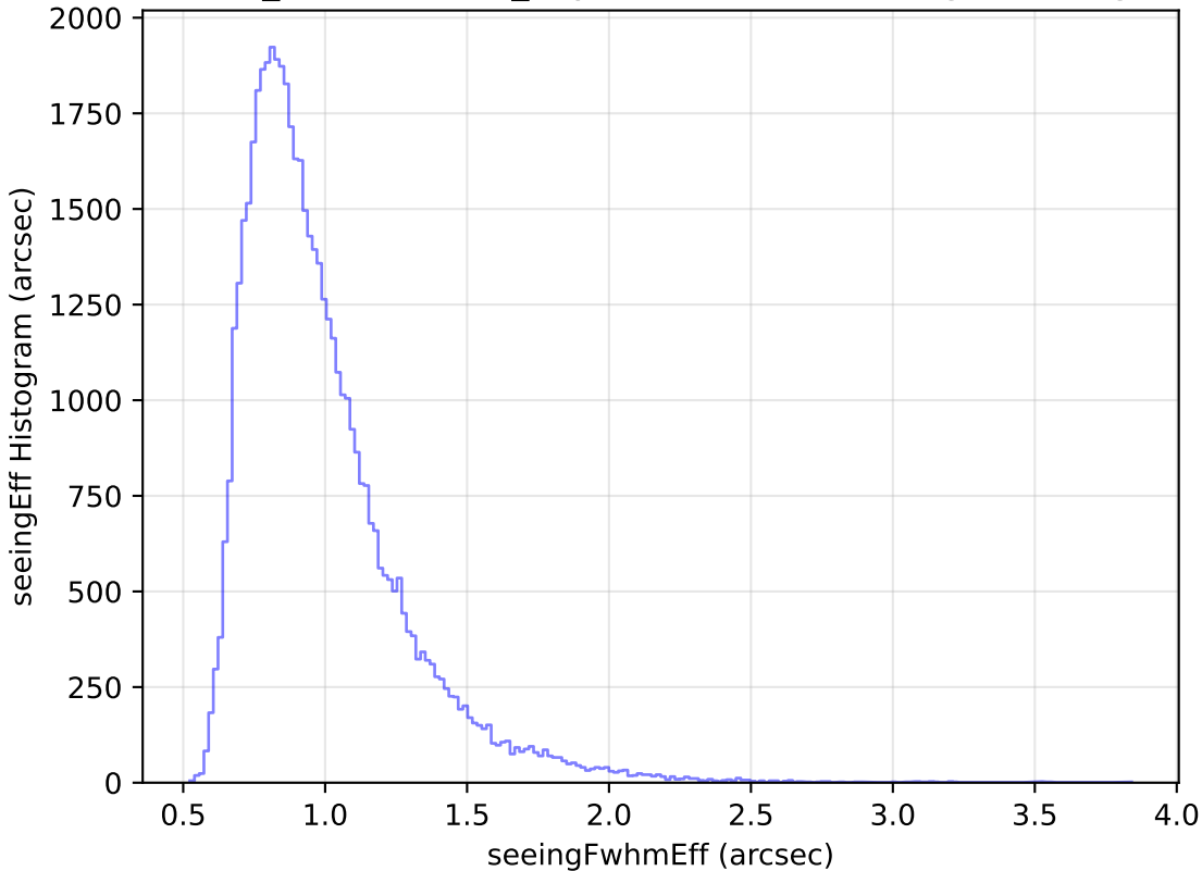
weather_cloudso6v3.4_10yrs Yr 1 i band: seeingEff Histogram
