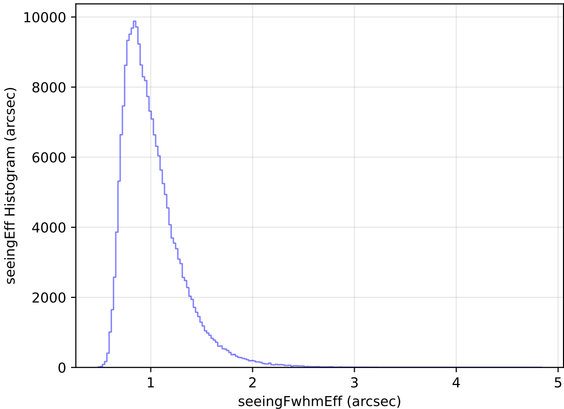
weather_cloudso6v3.4_10yrs Yr 1 all bands: seeingEff Histogram
