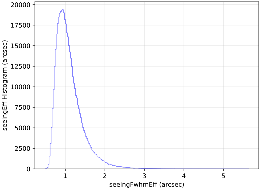
weather_cloudso6v3.4_10yrs WFD z band: seeingEff Histogram
