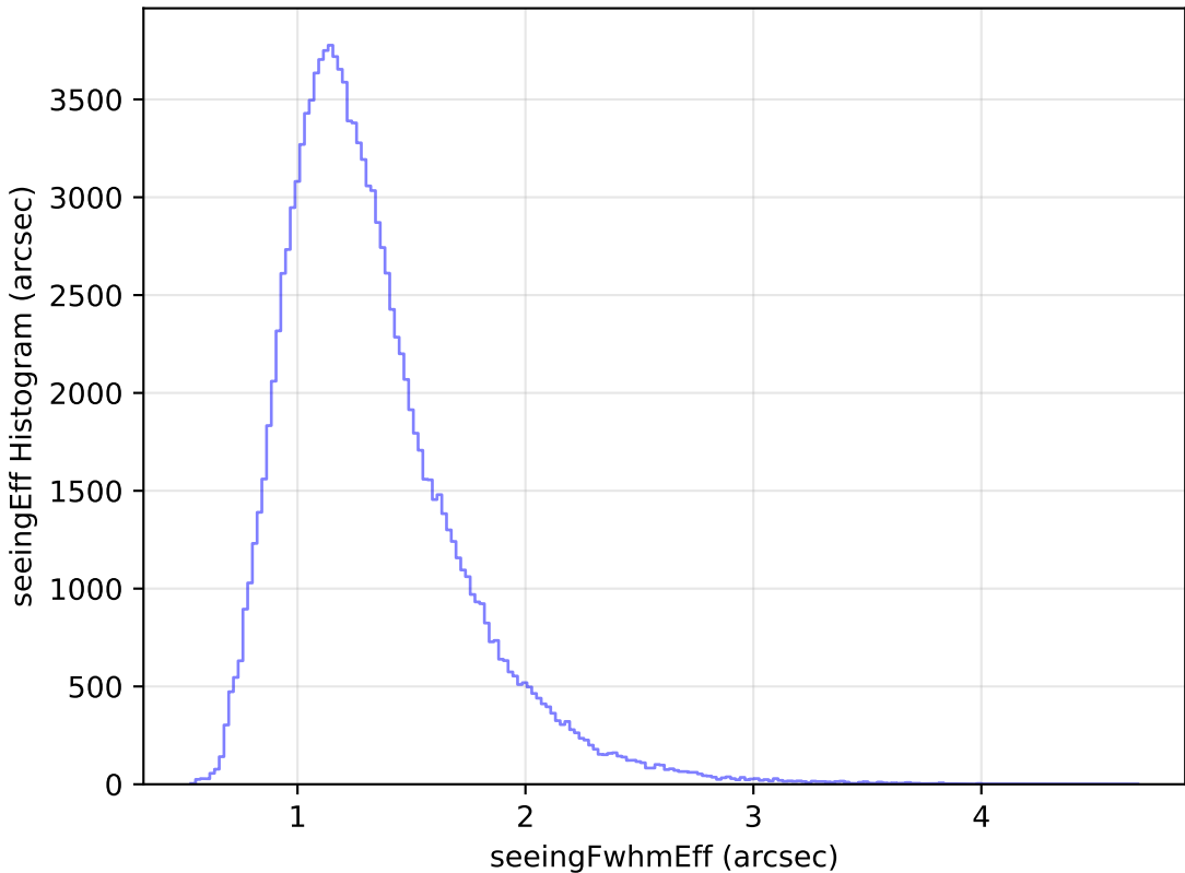
weather_cloudso6v3.4_10yrs WFD u band: seeingEff Histogram
