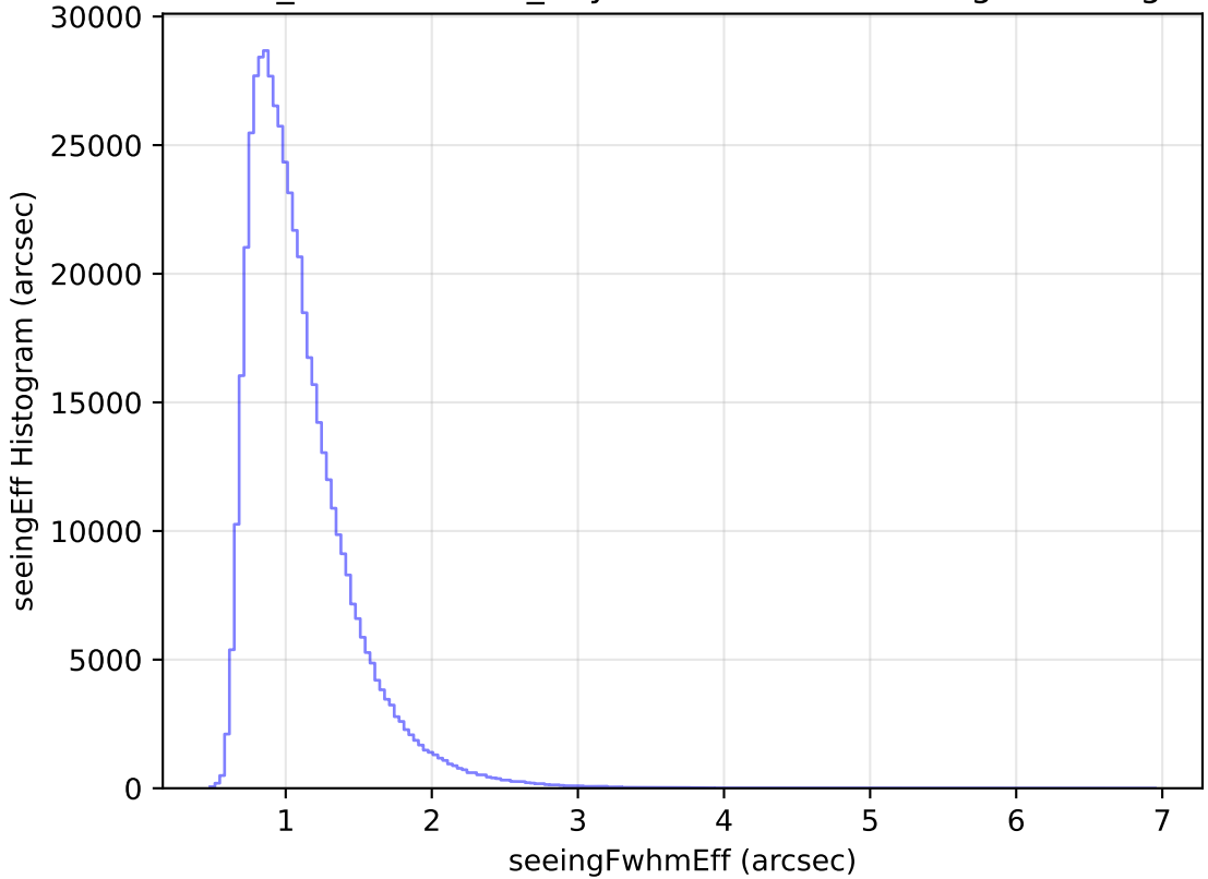
weather_cloudso6v3.4_10yrs WFD i band: seeingEff Histogram
