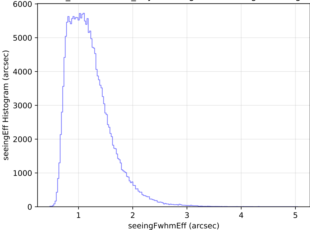
weather_cloudso6v3.4_10yrs WFD g band: seeingEff Histogram
