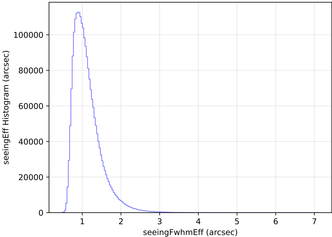
weather_cloudso6v3.4_10yrs WFD all bands: seeingEff Histogram
