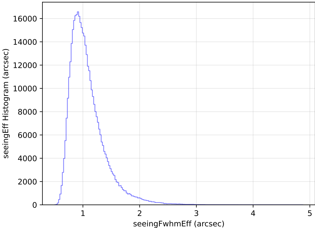
weather_cloudso6v3.4_10yrs All sky y band: seeingEff Histogram
