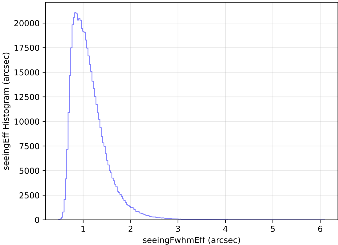
weather_cloudso6v3.4_10yrs All sky r band: seeingEff Histogram
