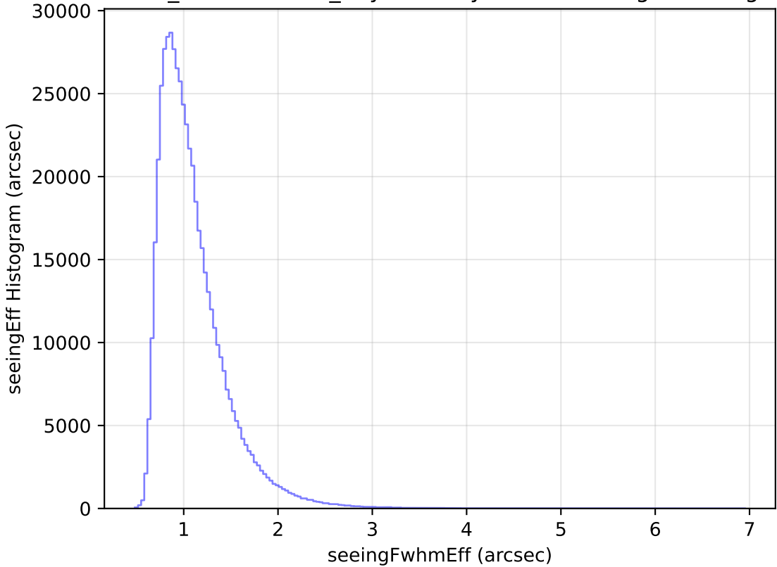
weather_cloudso6v3.4_10yrs All sky i band: seeingEff Histogram
