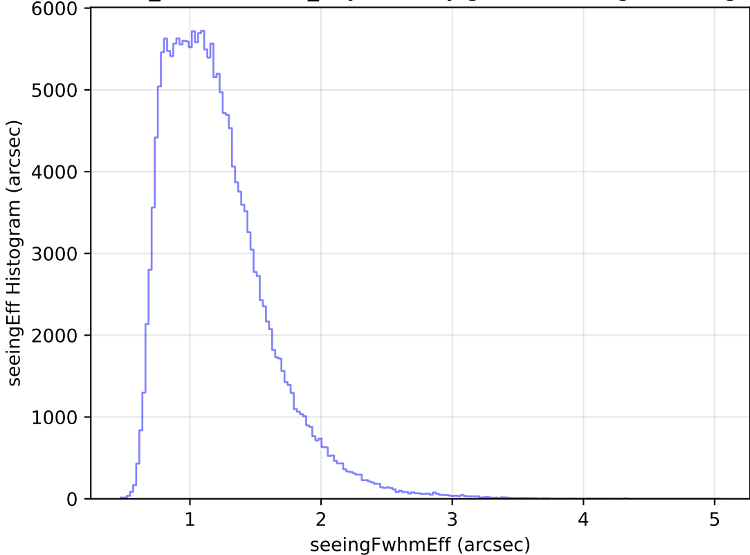
weather_cloudso6v3.4_10yrs All sky g band: seeingEff Histogram
