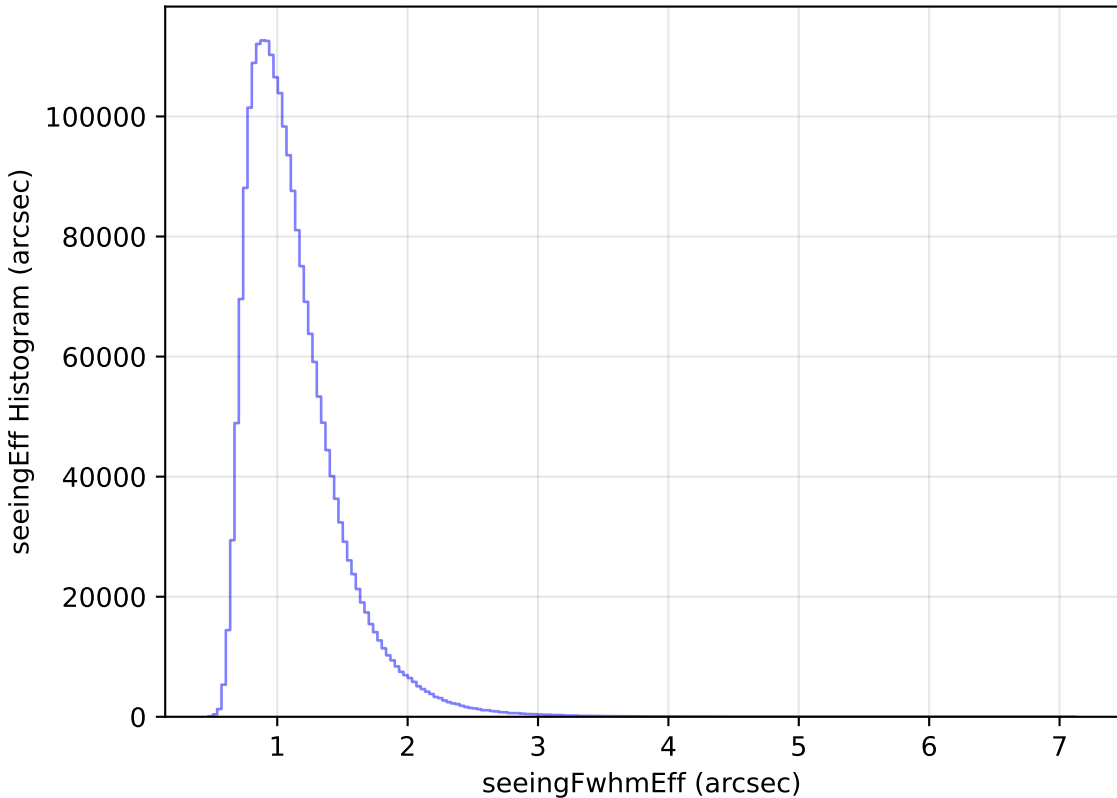
weather_cloudso6v3.4_10yrs All sky all bands: seeingEff Histogram
