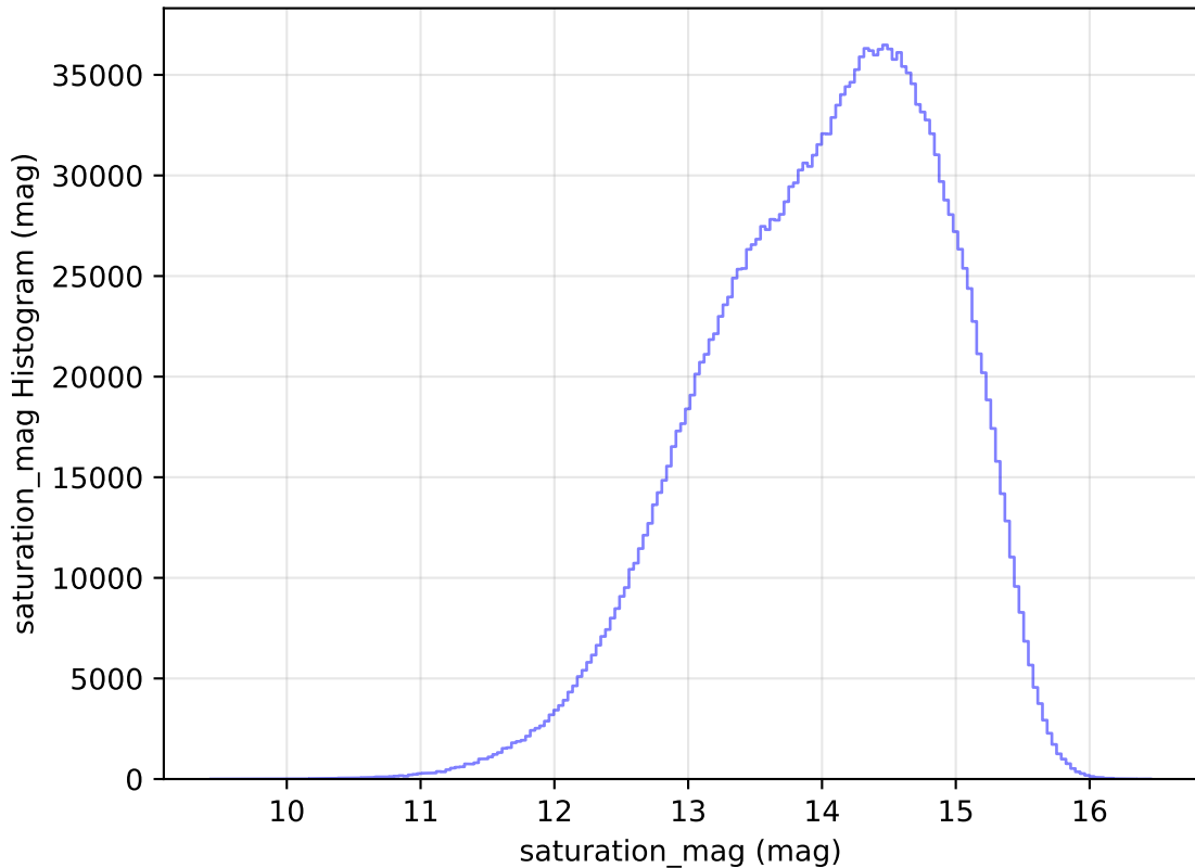
weather_cloudso6v3.4_10yrs WFD all bands: saturation_mag Histogram
