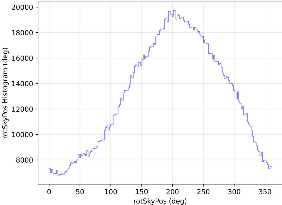
weather_cloudso6v3.4_10yrs All sky all bands: rotSkyPos Histogram
