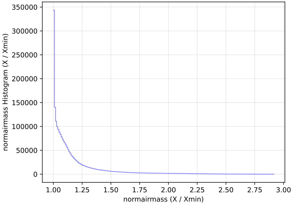
weather_cloudso6v3.4_10yrs WFD all bands: normairmass Histogram
