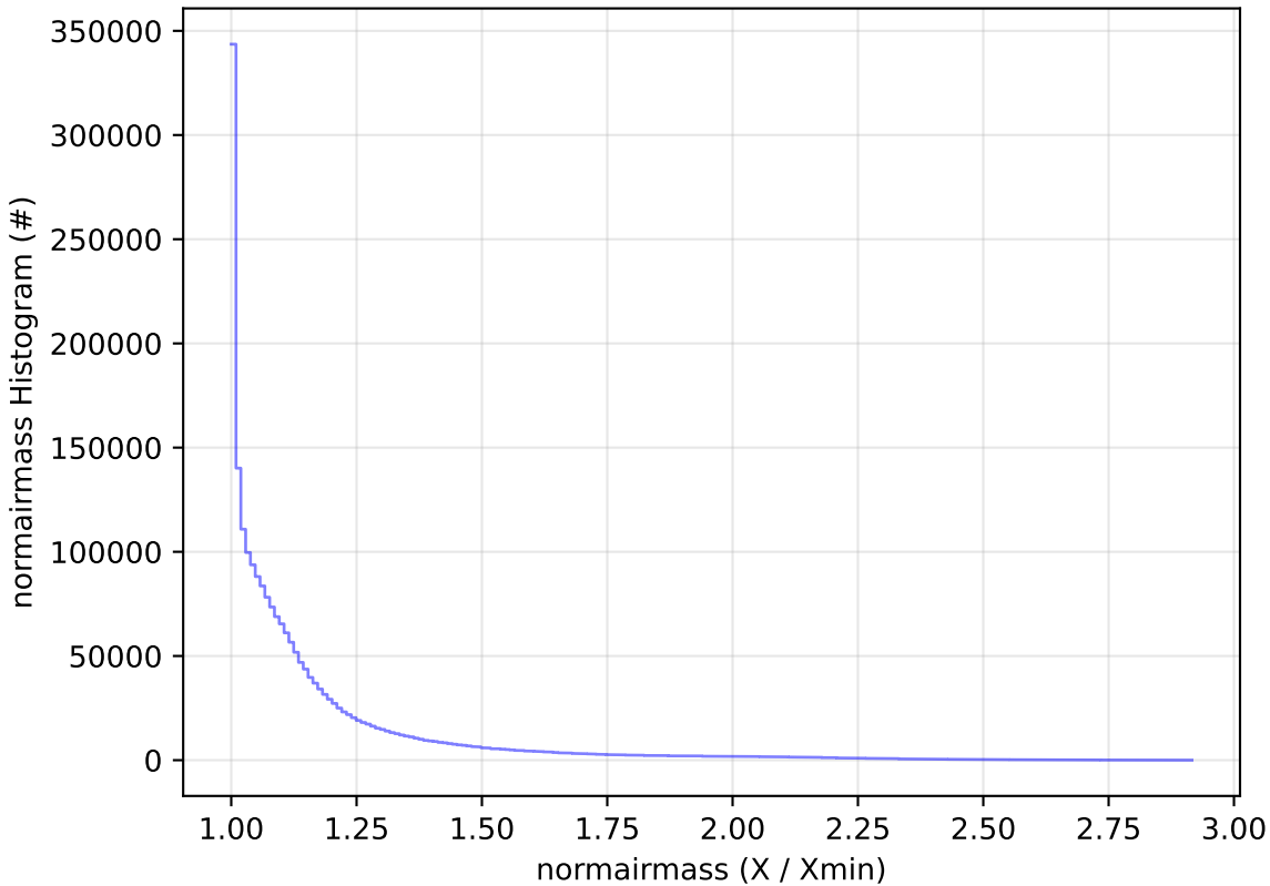
weather_cloudso6v3.4_10yrs All sky all bands: normairmass Histogram
