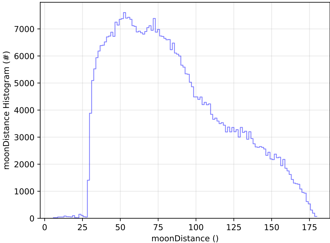
weather_cloudso6v3.4_10yrs WFD z band: moonDistance Histogram
