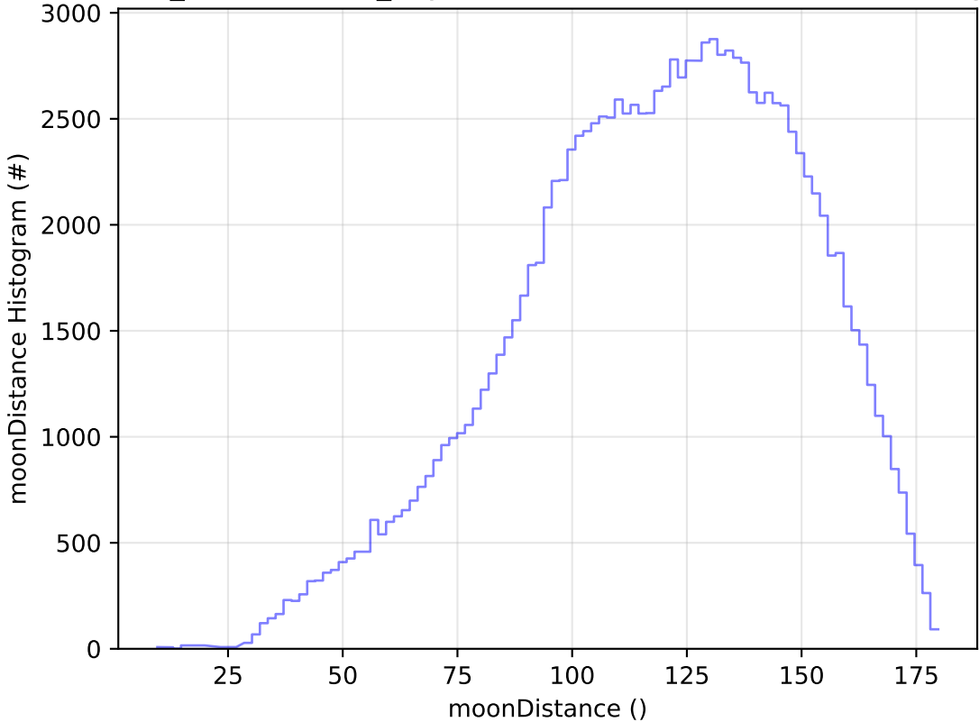
weather_cloudso6v3.4_10yrs WFD u band: moonDistance Histogram
