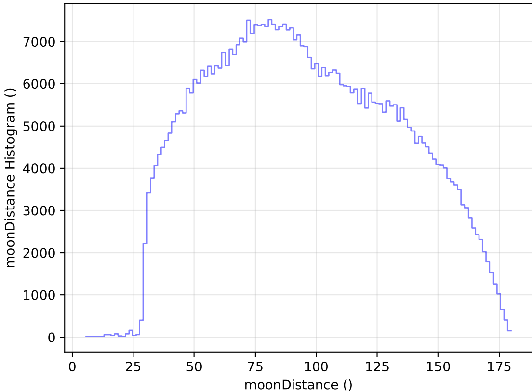
weather_cloudso6v3.4_10yrs WFD i band: moonDistance Histogram
