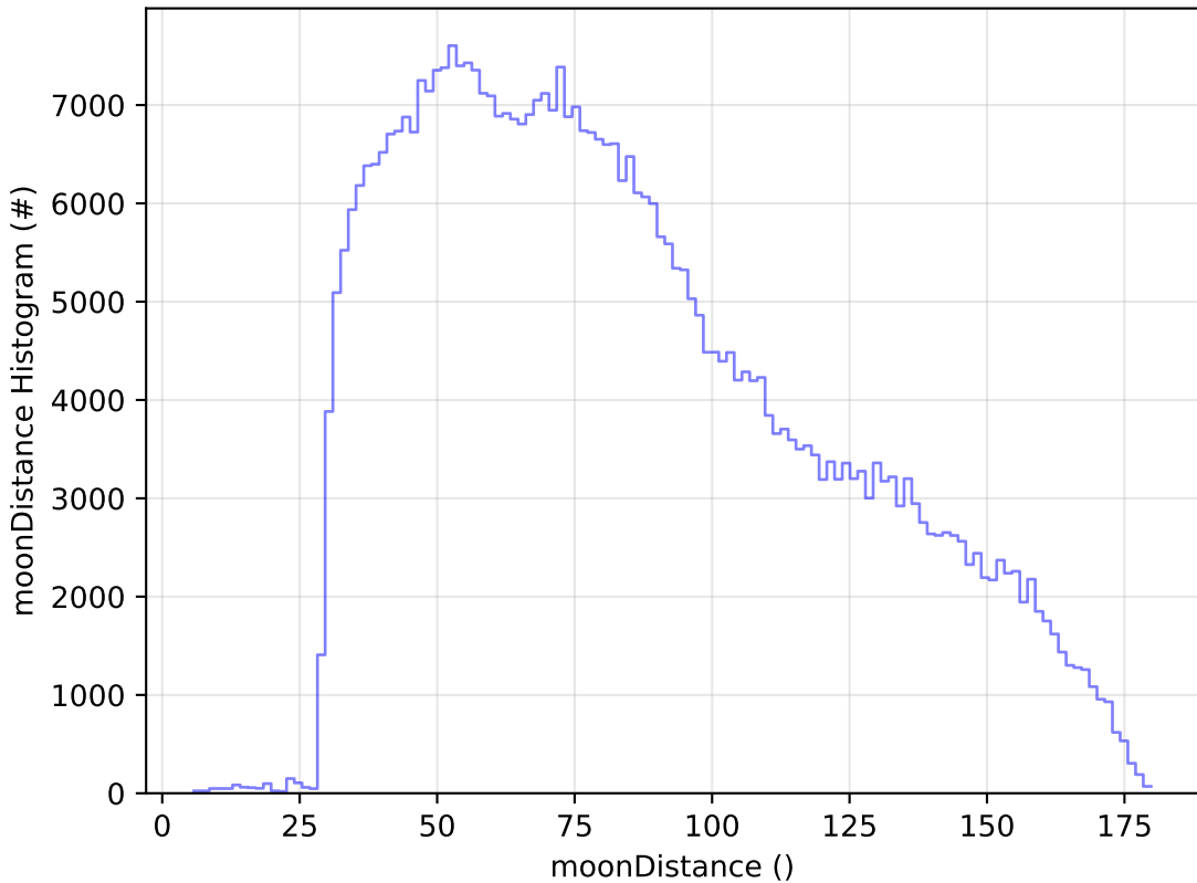
weather_cloudso6v3.4_10yrs All sky z band: moonDistance Histogram
