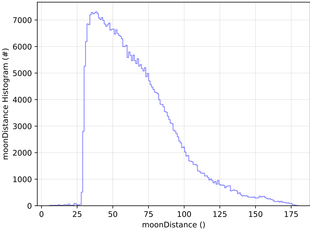
weather_cloudso6v3.4_10yrs All sky y band: moonDistance Histogram
