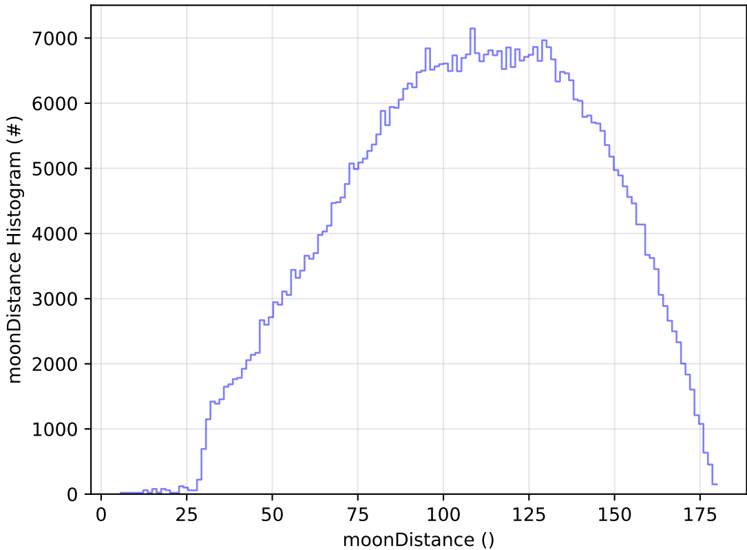
weather_cloudso6v3.4_10yrs All sky r band: moonDistance Histogram
