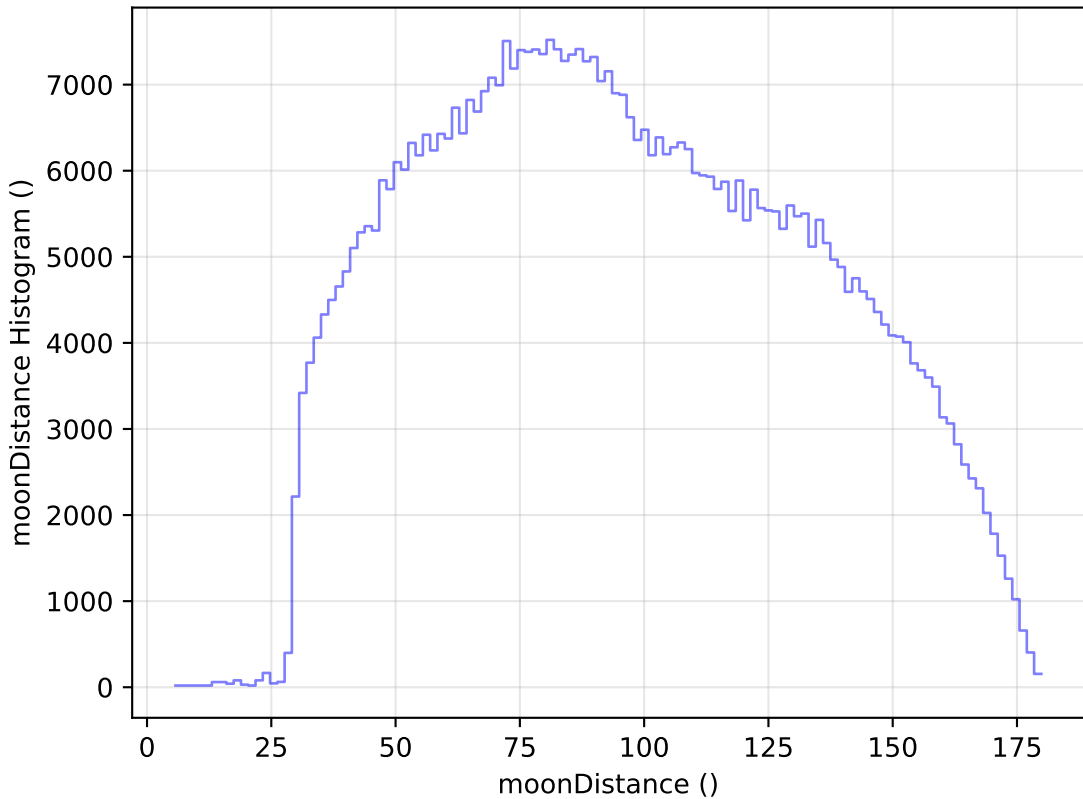
weather_cloudso6v3.4_10yrs All sky i band: moonDistance Histogram
