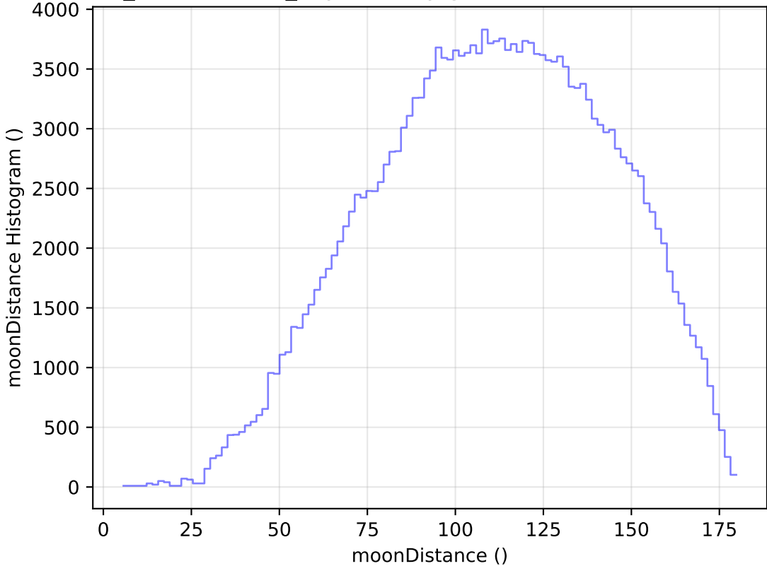
weather_cloudso6v3.4_10yrs All sky g band: moonDistance Histogram
