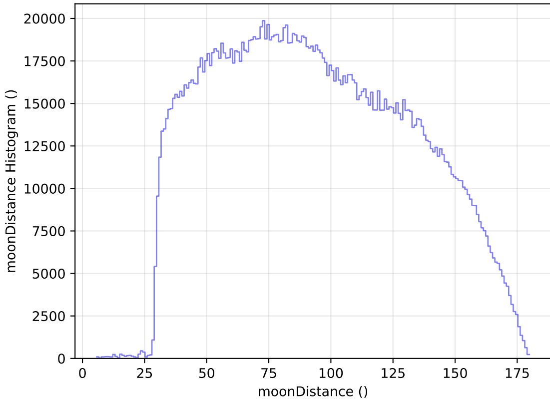
weather_cloudso6v3.4_10yrs All sky all bands: moonDistance Histogram
