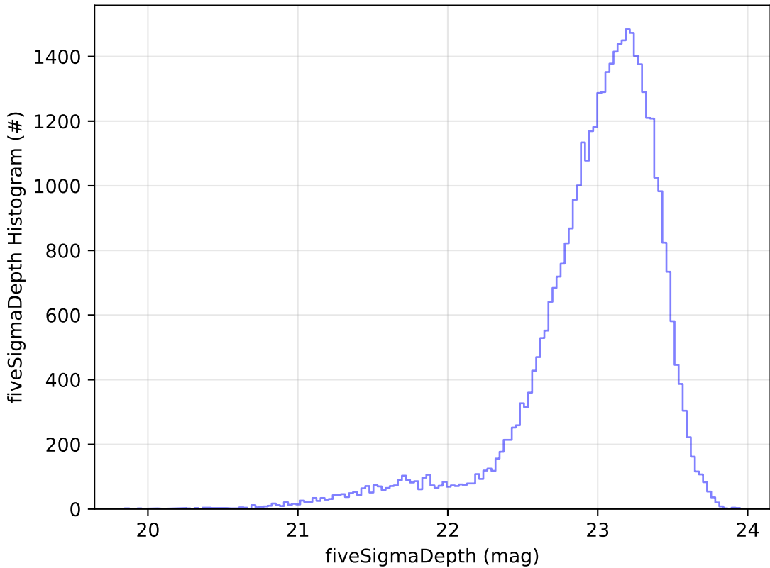
weather_cloudso6v3.4_10yrs Yr 1 z band: fiveSigmaDepth Histogram
