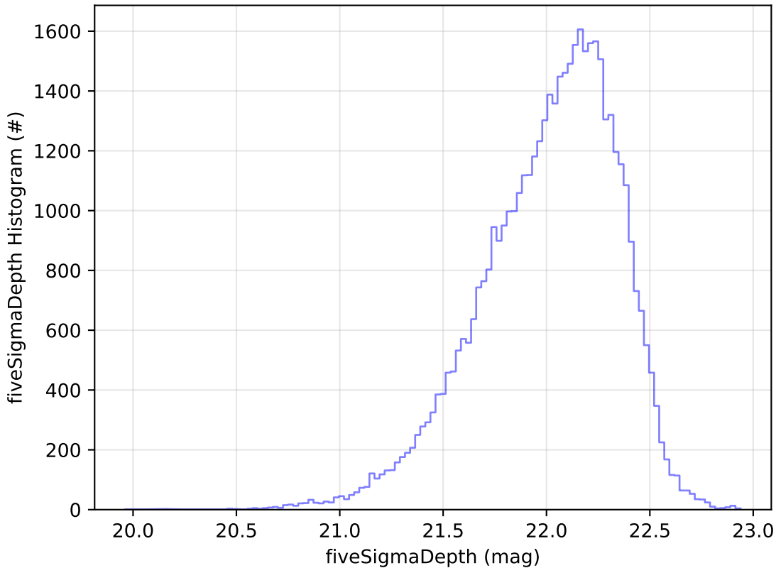
weather_cloudso6v3.4_10yrs Yr 1 y band: fiveSigmaDepth Histogram
