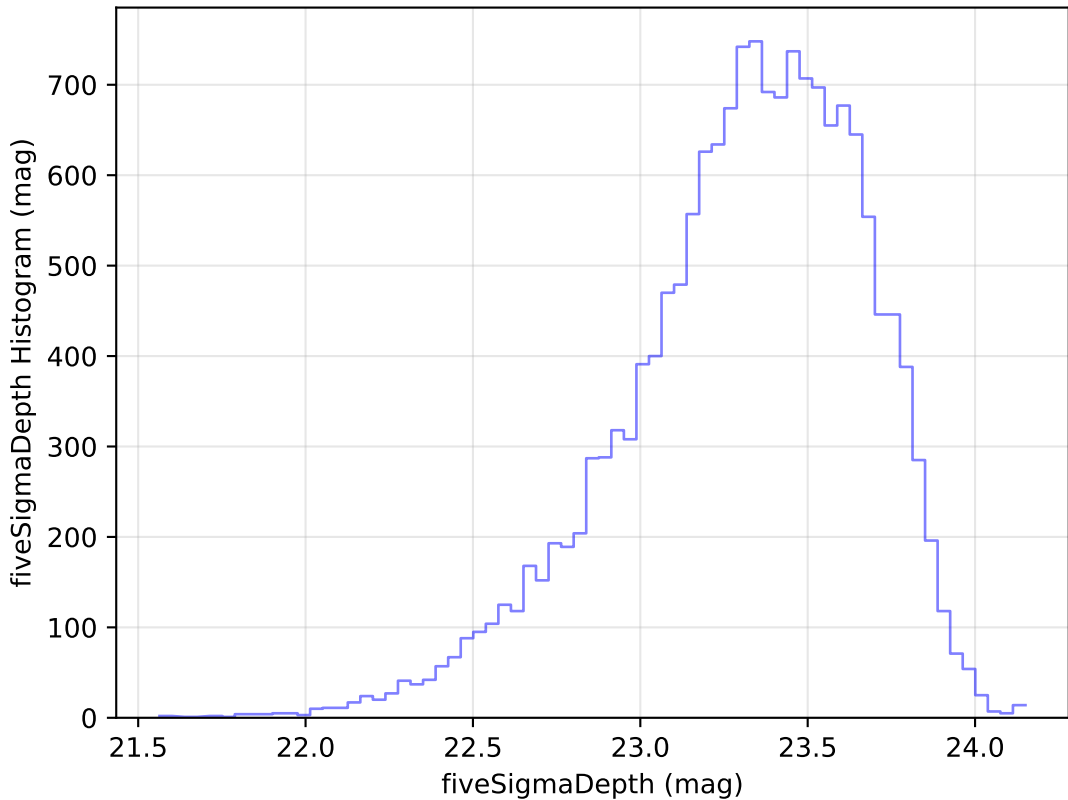
weather_cloudso6v3.4_10yrs Yr 1 u band: fiveSigmaDepth Histogram
