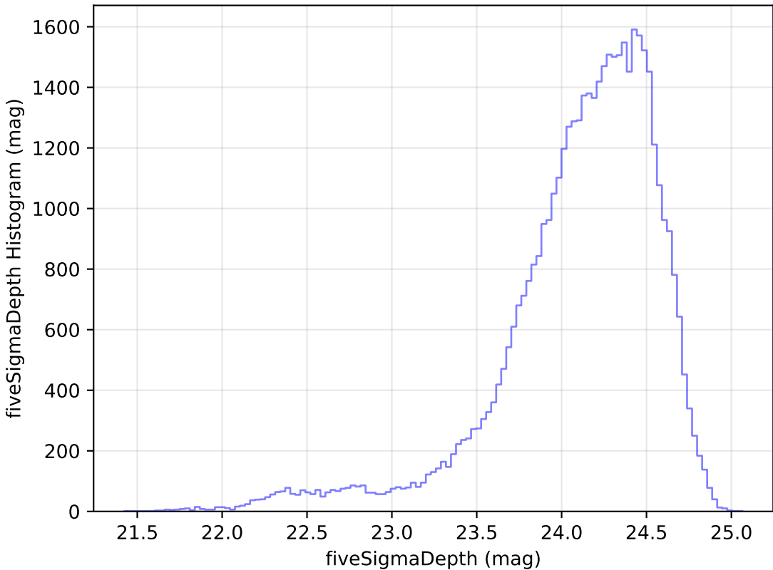
weather_cloudso6v3.4_10yrs Yr 1 r band: fiveSigmaDepth Histogram
