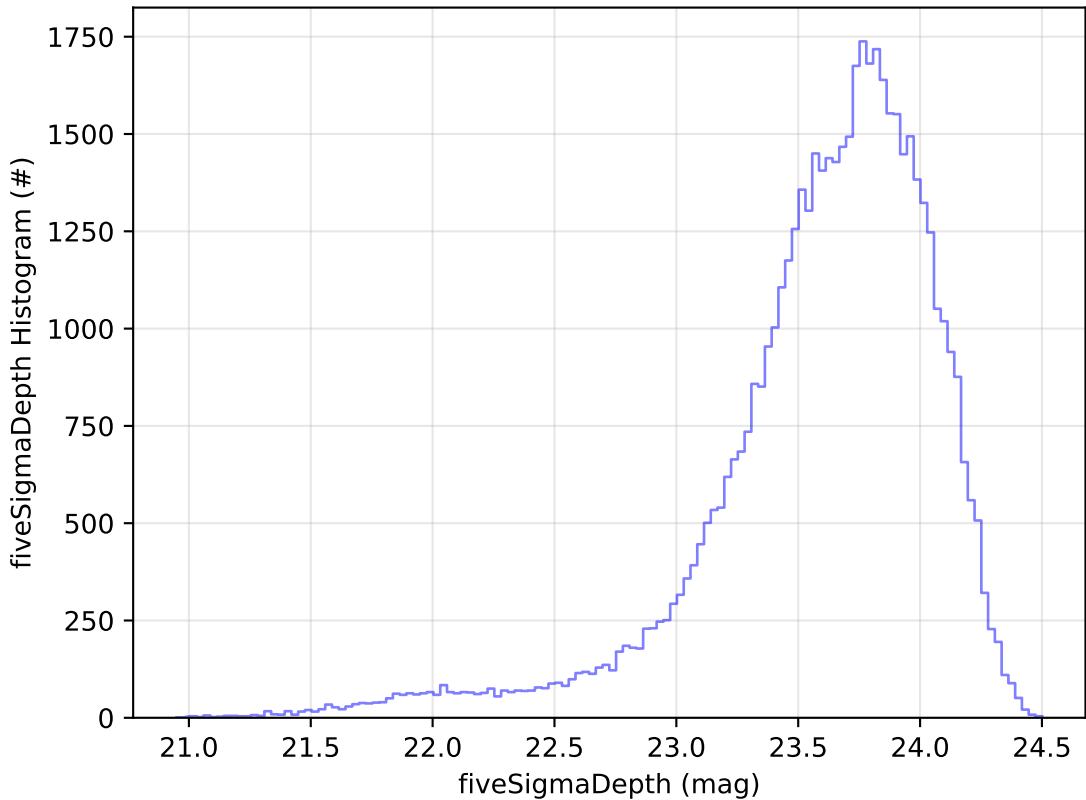
weather_cloudso6v3.4_10yrs Yr 1 i band: fiveSigmaDepth Histogram
