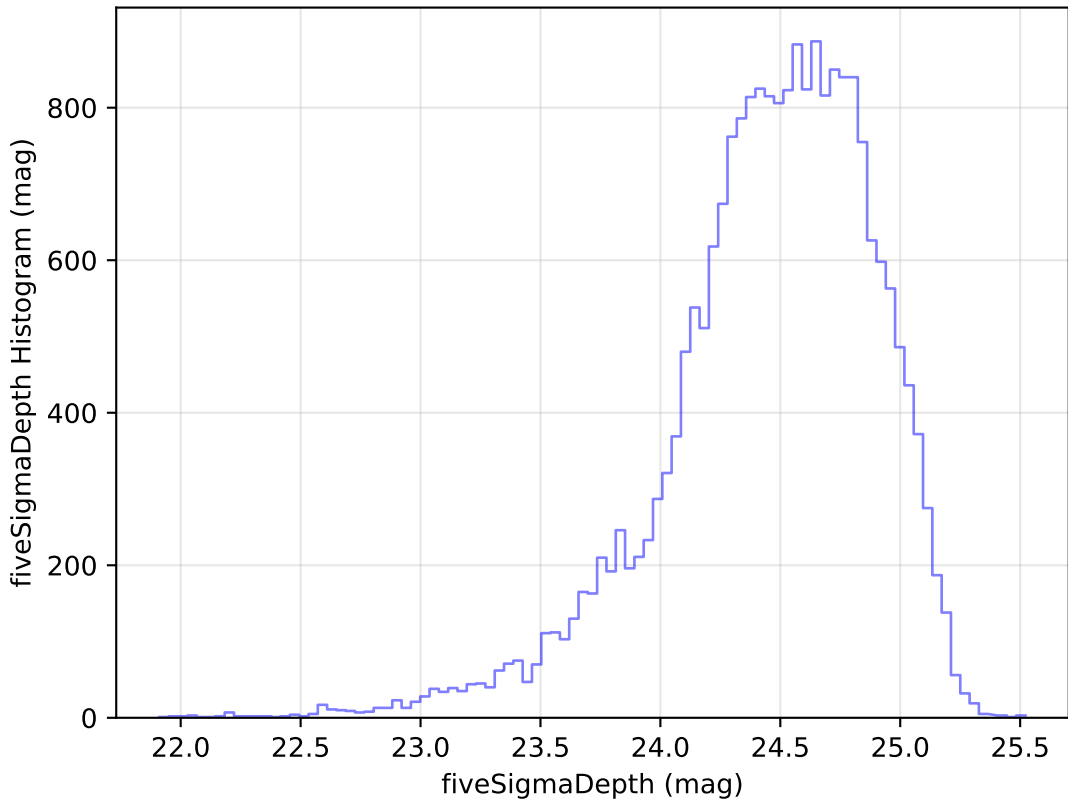
weather_cloudso6v3.4_10yrs Yr 1 g band: fiveSigmaDepth Histogram
