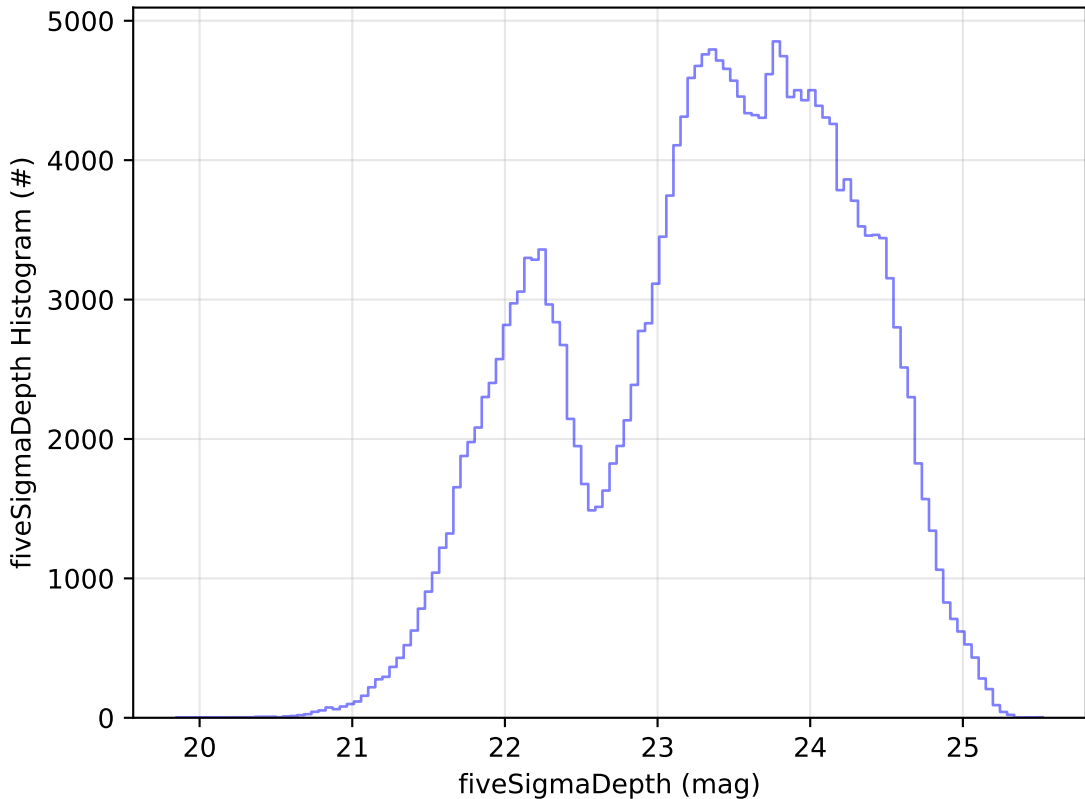
weather_cloudso6v3.4_10yrs Yr 1 all bands: fiveSigmaDepth Histogram
