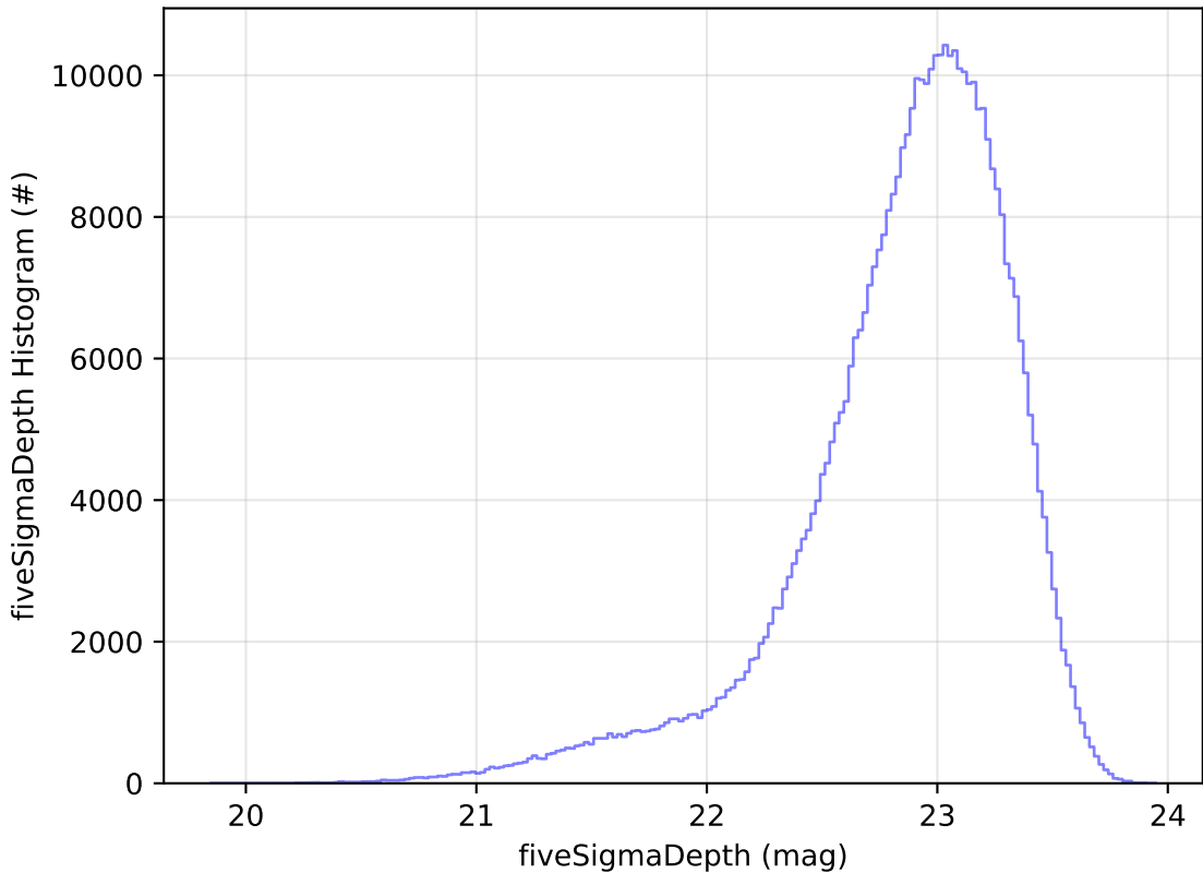
weather_cloudso6v3.4_10yrs WFD z band: fiveSigmaDepth Histogram
