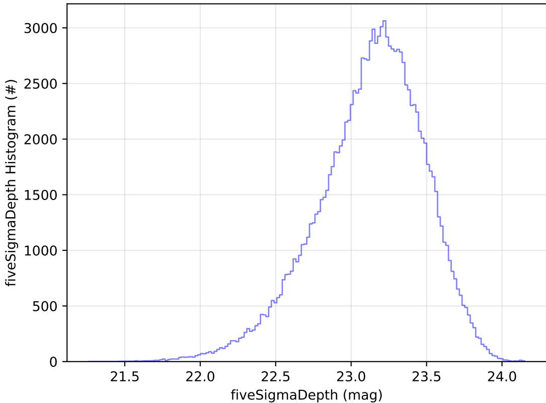
weather_cloudso6v3.4_10yrs WFD u band: fiveSigmaDepth Histogram
