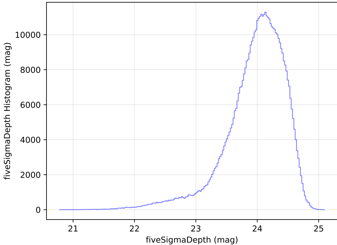
weather_cloudso6v3.4_10yrs WFD r band: fiveSigmaDepth Histogram
