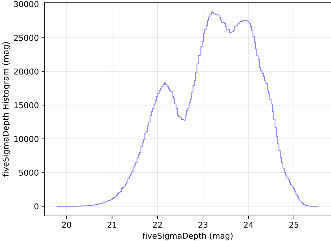
weather_cloudso6v3.4_10yrs WFD all bands: fiveSigmaDepth Histogram
