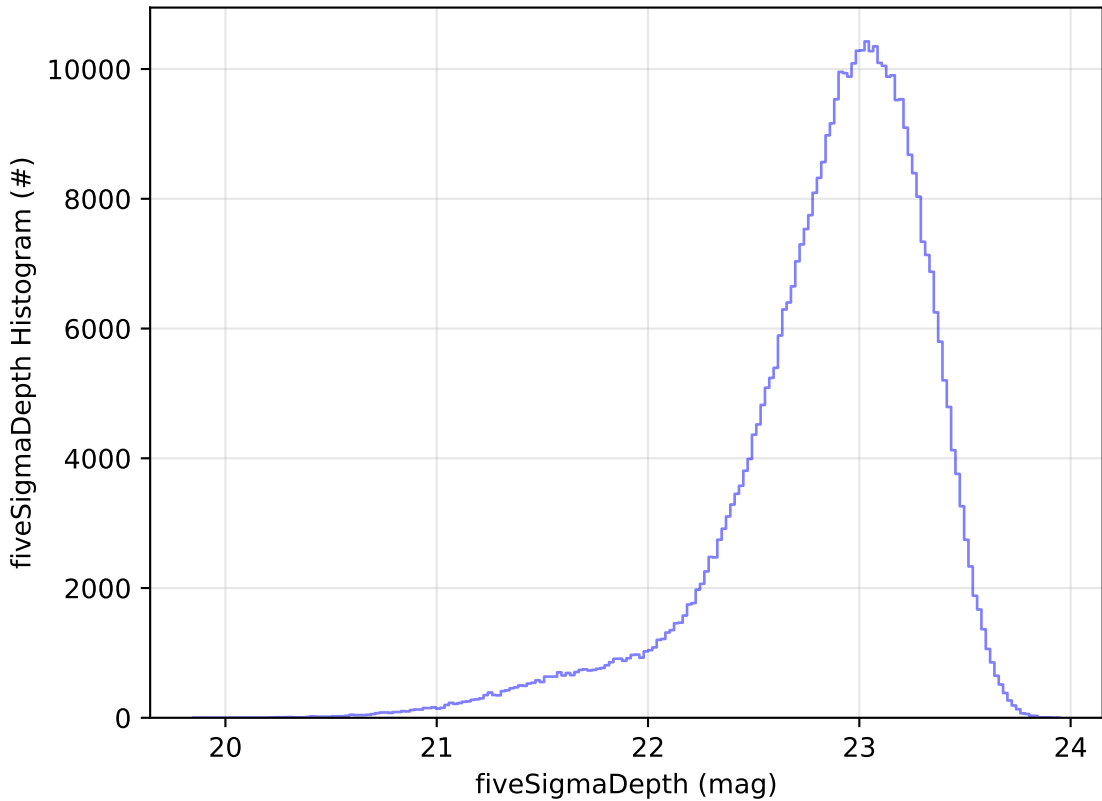
weather_cloudso6v3.4_10yrs All sky z band: fiveSigmaDepth Histogram
