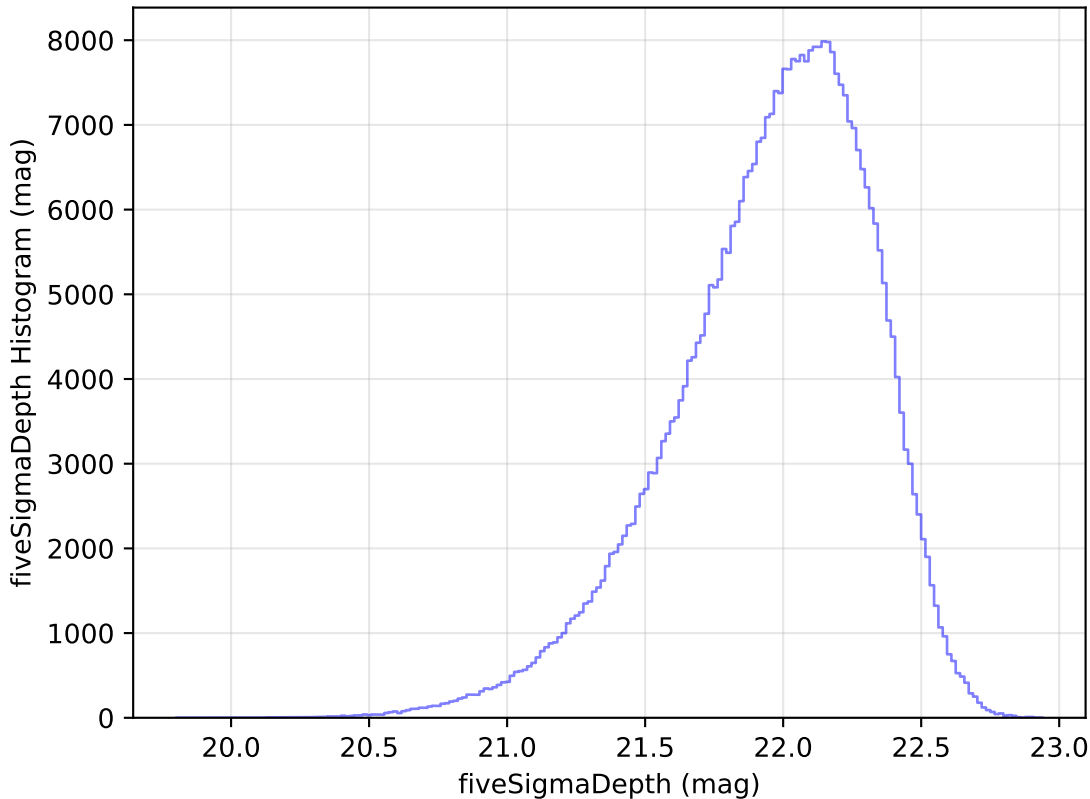
weather_cloudso6v3.4_10yrs All sky y band: fiveSigmaDepth Histogram
