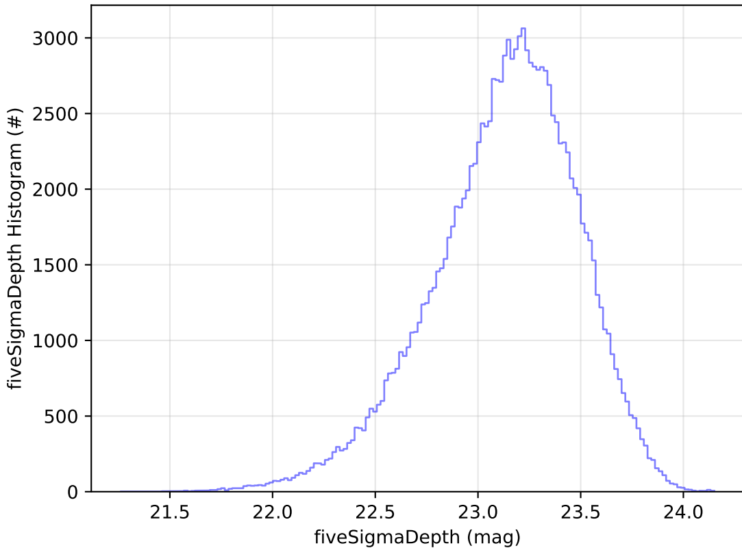
weather_cloudso6v3.4_10yrs All sky u band: fiveSigmaDepth Histogram
