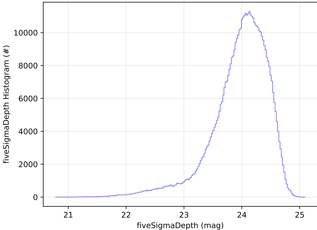
weather_cloudso6v3.4_10yrs All sky r band: fiveSigmaDepth Histogram
