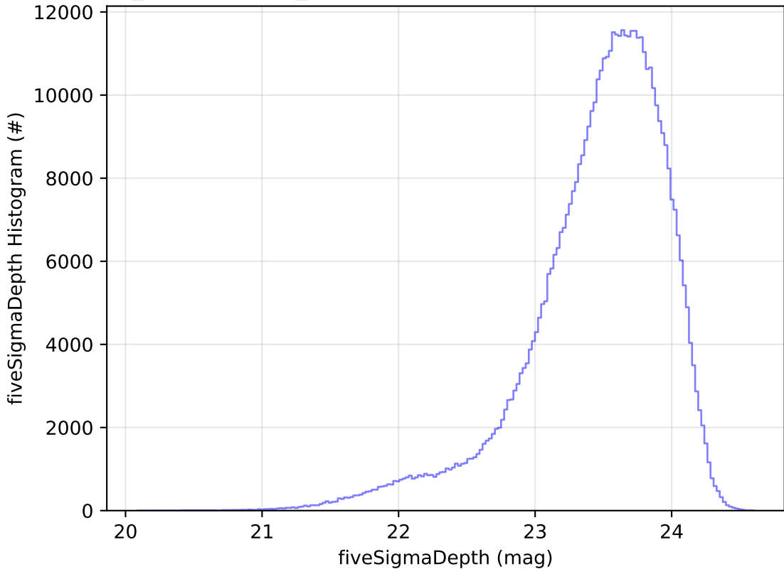
weather_cloudso6v3.4_10yrs All sky i band: fiveSigmaDepth Histogram
