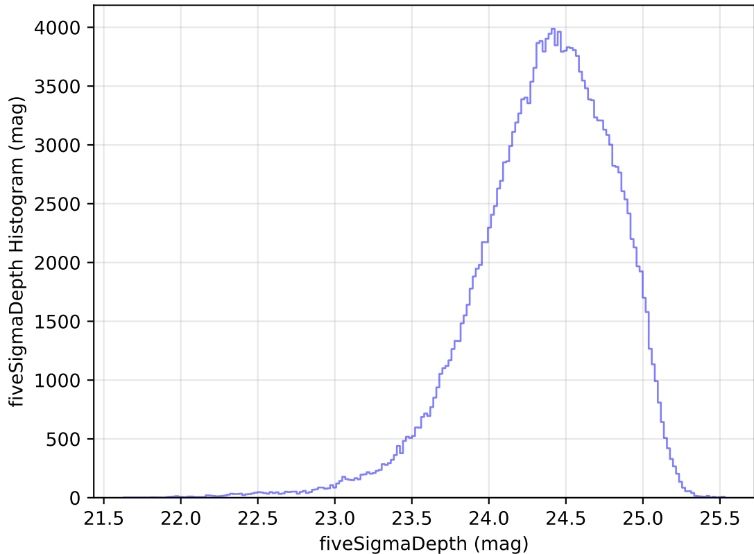
weather_cloudso6v3.4_10yrs All sky g band: fiveSigmaDepth Histogram
