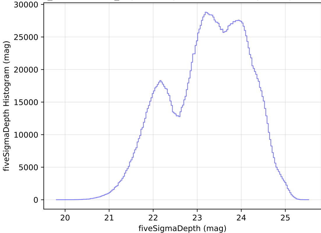
weather_cloudso6v3.4_10yrs All sky all bands: fiveSigmaDepth Histogram
