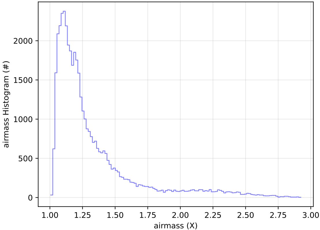
weather_cloudso6v3.4_10yrs Yr 1 z band: airmass Histogram
